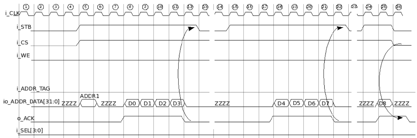
Figure 6: Multiblock write transaction on the processor bus
