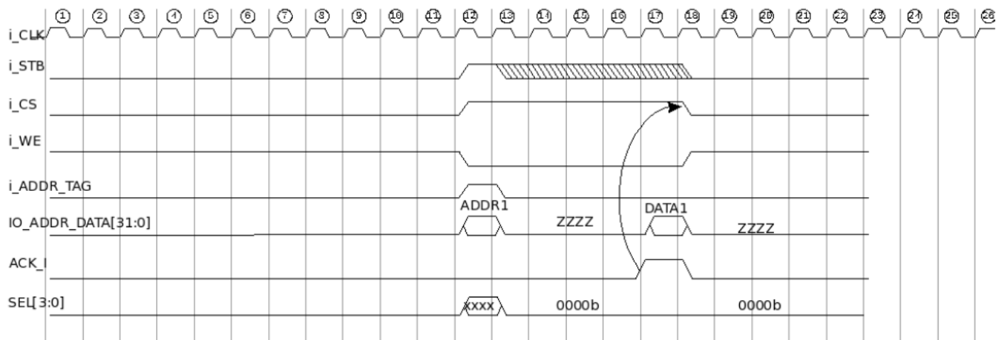
Figure 3: Single word read cycle on the processor interface
